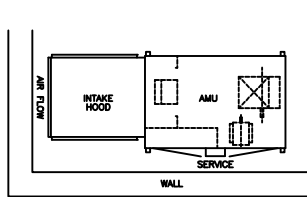
INCORRECT NO AIR FLOW OR SERVICE CLEARANCE
