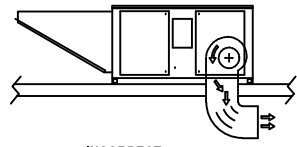
INCORRECT ADDS HIGH AMOUNT OF STATIC PRESSURE ELBOW TOO CLOSE TO DISCHARGE
