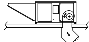
CORRECT USE A 45° DIFFUSER, STRAIGHT DIFFUSER, OR INCREASE DISTANCE TO ELBOW **SEE DUCTWORK CHART**
