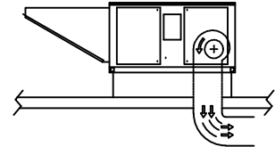
CORRECT USE RADIUS ELBOWS WITH TURNING VANES
