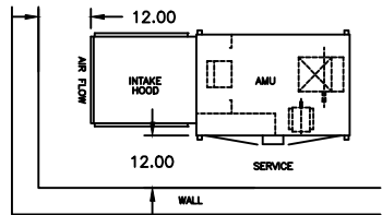
CORRECT 24.00" MINIMUM SERVICE CLEARANCE
